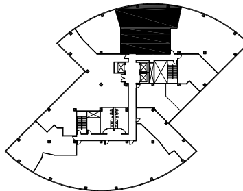
6TH FLOOR
